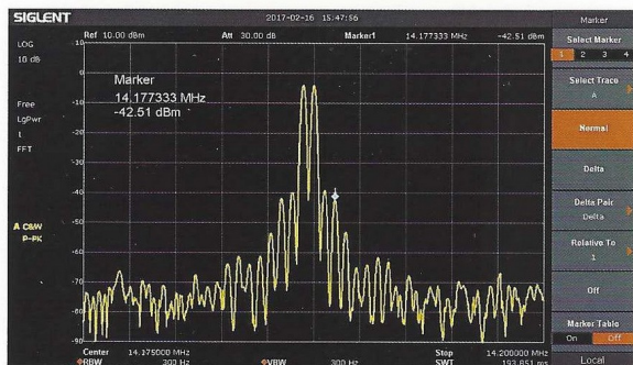
IMD on 14Mhz
